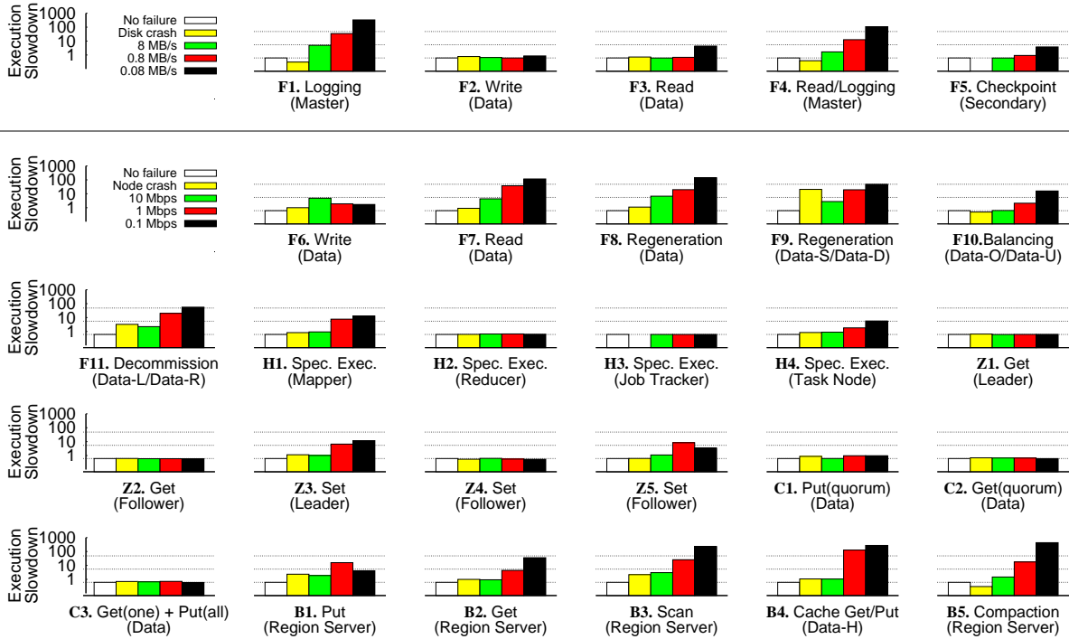
Figure 1: Limpbench Results. Each graph represents the result of each experiment (e.g., F1) described in Table 1. The y-axis plots the slowdowns (in log scale) of an experiment under various limpware scenarios. In the first row, a slow disk is injected. In the rest, a slow NIC is injected. The graphs show that cloud systems are crash tolerant, but not limpware tolerant.
